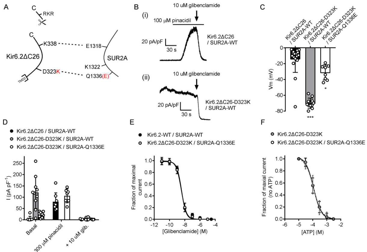
Figure 10: Kir6.2ΔC26-D323K co-expression with SUR2A-Q1336E restores sulphonylurea sensitivity however the channel remains partially constitutively active
