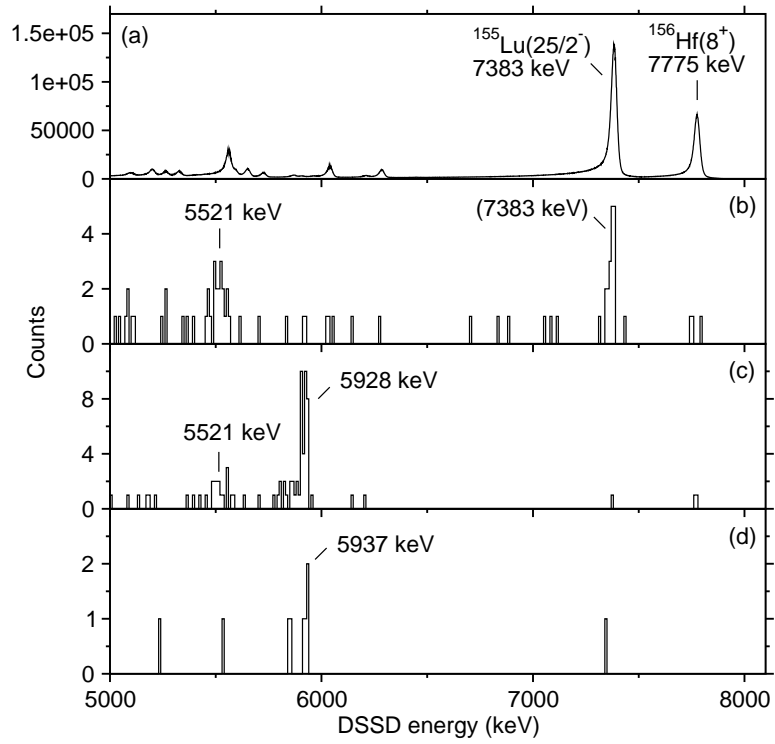
FIG. 2: DSSD \alpha -particle energy spectra recorded up to 8.2 ms after a recoil implantation was identified in the same DSSD pixel. Panel (a) shows all \alpha -particle energies. The other panels show \alpha -particle energies in coincidence with 415- (b), 1490- (c) and 1478-keV (d) \gamma rays from ^{151}\text{Tm} .
