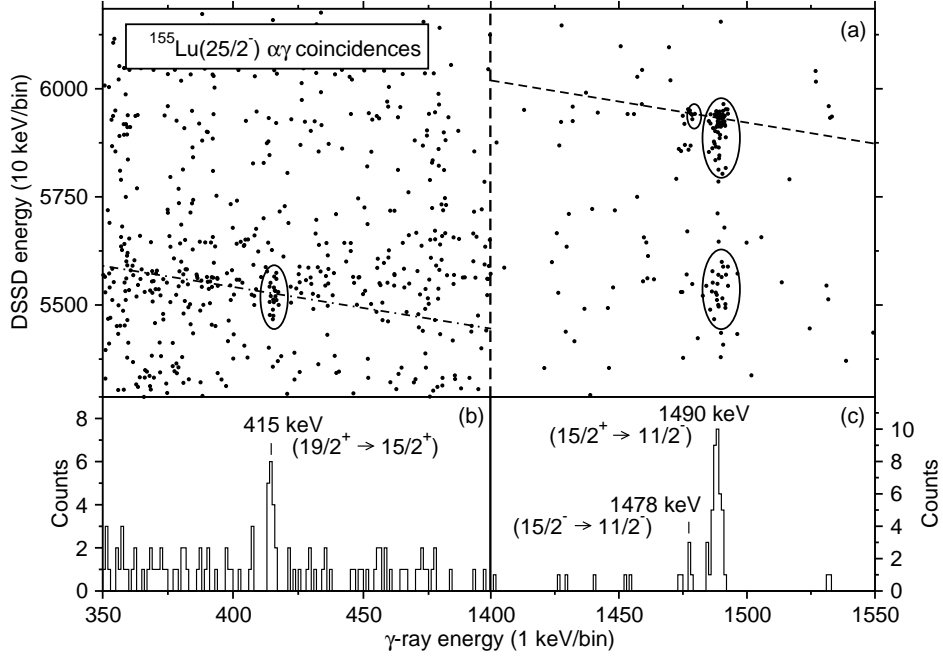
FIG. 4: Energies of coincident \alpha particles and \gamma rays measured following the decay of ^{155}\text{Lu}(25/2^-) . The diagonal lines on Panel (a) represent a constant energy for the sum of the \alpha -decay Q value, calculated from the \alpha -particle energy, and the \gamma -ray energy; the energies represented are those between the ^{155}\text{Lu}(25/2^-) isomeric state and both the ground state (dashed line) and excited state at 1490 keV (dot-dashed line) in ^{151}\text{Tm} . The \alpha\gamma coincidences identified are circled and the \gamma -ray projections in coincidence with the 5521(8)-keV (b) and the 5928(5)- or 5937(15)-keV (c) \alpha particles are shown.
