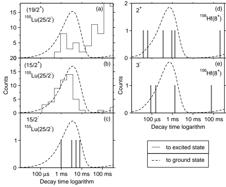
FIG. 3: Decay times for the \alpha decay identified from ^{155}\text{Lu}(25/2^-) to the (19/2^+) (a), (15/2^+) (b) and 15/2^- (c) states in ^{151}\text{Tm} and from ^{156}\text{Hf}(8^+) to the 2^+ (d) and 3^- (e) states in ^{152}\text{Yb} . Also shown as a dashed line on each panel is the distribution of the decay times from the respective isomer to the ground state. These have been scaled for comparison with the weaker branches.
