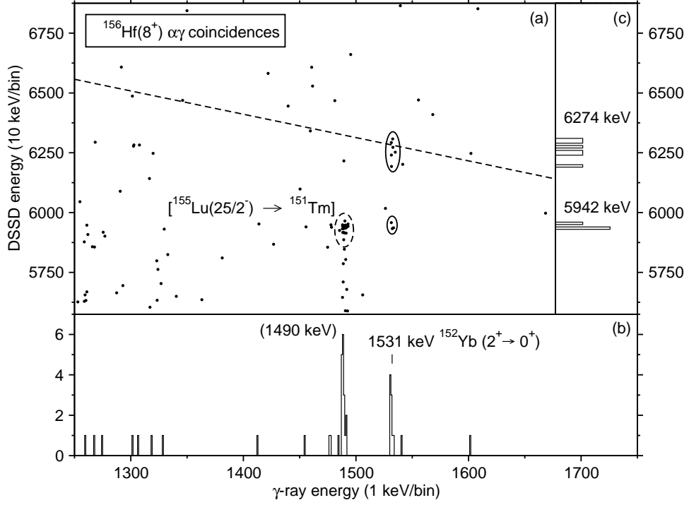
FIG. 5: Energies of coincident \alpha particles and \gamma rays measured following the decay of ^{156}\text{Hf}(8^+) . The diagonal line on Panel (a) represents a constant energy for the sum of the \alpha -decay Q value, calculated from the \alpha -particle energy and the \gamma -ray energy; the energy represents that between the ^{156}\text{Hf}(8^+) isomeric state and the ground state of ^{152}\text{Yb} . The \alpha\gamma coincidences identified from ^{156}\text{Hf}(8^+) are circled with contaminant coincidences from ^{155}\text{Lu}(25/2^-) also labelled. Also shown are the \gamma -ray energies in coincidence with the 5942(15)- or 6274(15)-keV \alpha particles (b) and the \alpha -particle energies in coincidence with the 1531-keV \gamma rays (c).
