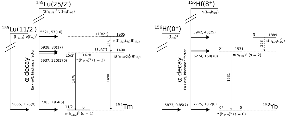
FIG. 1: Level schemes of ^{151}\text{Tm} and ^{152}\text{Yb} populated following the \alpha decays of the ^{155}\text{Lu} J^\pi = 25/2^- isomer and ground state and the ^{156}\text{Hf} J^\pi = 8^+ isomer and ground state, respectively. The spins, parities and energies of each level are given along with the energies of the transitions. For each \alpha decay the \alpha -particle energy and reduced hindrance factors are given and the state populated is indicated. The configurations which have previously been assigned to each state (see text for details) are shown.
