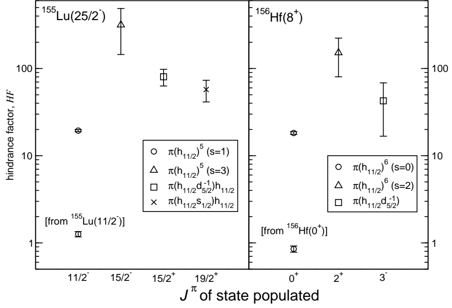
FIG. 6: Reduced hindrance factors of the \alpha decays from the ^{155}\text{Lu}(25/2^-) and ^{156}\text{Hf}(8^+) isomers (except where labelled) to states in ^{151}\text{Tm} and ^{152}\text{Yb} , respectively, with J^\pi shown on the x axis. The configurations assigned to each of the states populated is indicated and analogous states in ^{151}\text{Tm} and ^{152}\text{Yb} have the same symbols.
