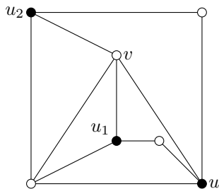
Figure 1. An example of a 4P_1 -free near-bipartite graph G with \text{ifvs}(G) = \text{fvs}(G) + 1 .
