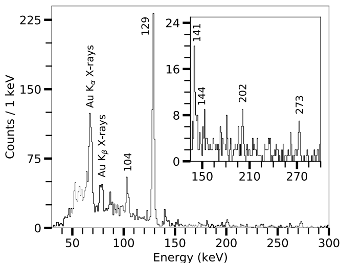
FIG. 3. The \gamma -ray energy spectrum with an energy gate on the 4550 to 6500 keV \alpha particles and a coincidence time gate 70\text{ns} \leq \Delta T(\gamma-\alpha) \leq 300\text{ns} . An expanded view of the spectrum between 135 keV and 300 keV is shown in the inset. Peaks are labeled according to corresponding transition energy in keV.
