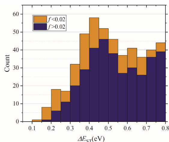
Fig. 2 The number of molecules in different range of energy gap. The blue and orange bars denote the number of the molecules with f > 0.02 and f < 0.02 , respectively.
