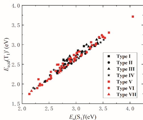
Fig. 3 The calibrated excitation energies of E_0(\text{S}_1) and E_0(\text{T}_1) for the selected 125 candidates.
