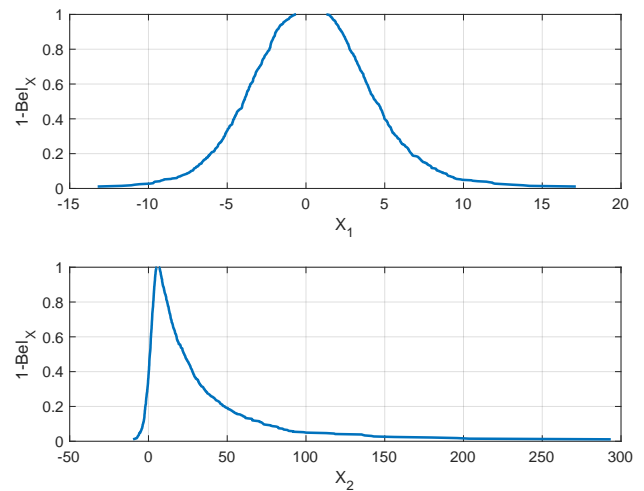
Figure 2: Plausibility contours obtained from Eqs.5 and 6, projecting onto the coordinate axes.
