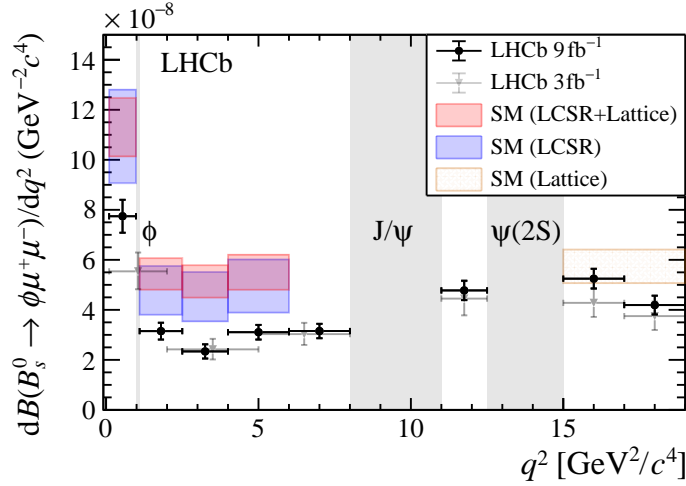
Figure 2: Differential branching fraction d\mathcal{B}(B_s^0 \rightarrow \phi\mu^+\mu^-)/dq^2 , overlaid with SM predictions using Light Cone Sum Rules [32, 34, 35] at low q^2 and Lattice calculations [36, 37] at high q^2 . The results from the LHCb 3 fb -1 analysis [1, 30] are shown with gray markers.
