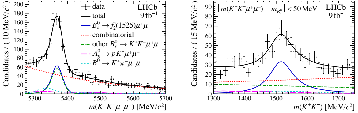
Figure 3: Reconstructed invariant mass of (left) the K^+K^-\mu^+\mu^- system and (right) the K^+K^- system for B_s^0 \rightarrow f_2'(1525)\mu^+\mu^- candidates, overlaid with the fit projections. The m(K^+K^-) distribution is shown in the B_s^0 signal region \pm 50 \text{ MeV}/c^2 around the known B_s^0 mass.
