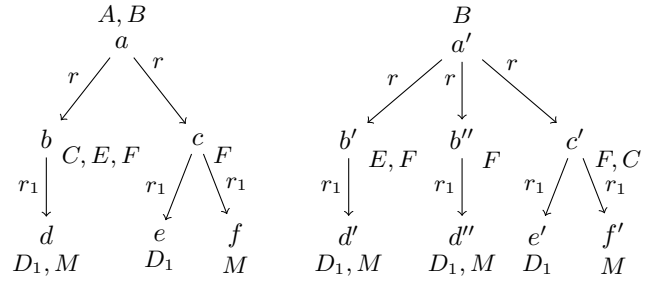
Figure 5: Interpretations \mathcal{I} (left) and \mathcal{I}' (right).
