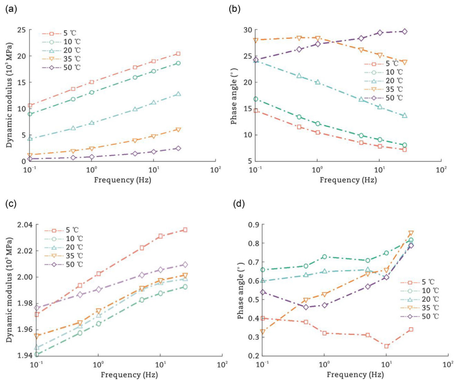
Fig. 63. Experimental results at different frequencies and temperatures. (a) Dynamic modulus of SMA-13. (b) Phase angle of SMA-13. (c) Dynamic modulus of ABS. (d) Phase angle of ABS (Jiang et al., 2023b).
