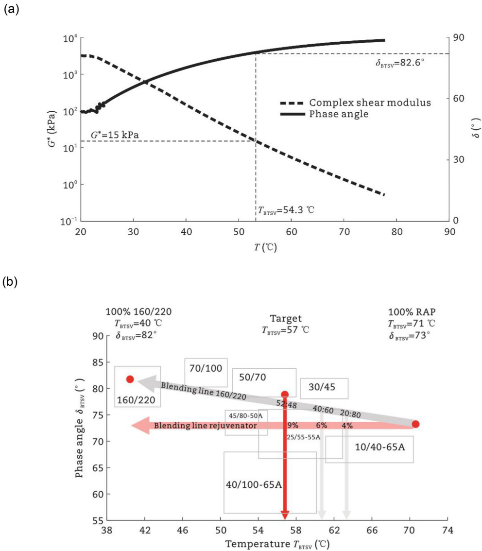
Fig. 14. Illustration of BTVS method and BTVS plane. (a) Example for BTVS method to determine softening temperature T_{BTSV} and corresponding phase angle \delta_{BTSV} . (b) BTVS plane and illustration of recycled binders blending with soft binder and rejuvenator (Alisov et al., 2020).
