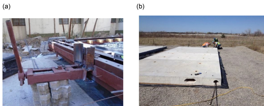
Fig. 56. Typical application of prestress slab system. (a) Pre-tensioning. (b) Post-tensioning.
