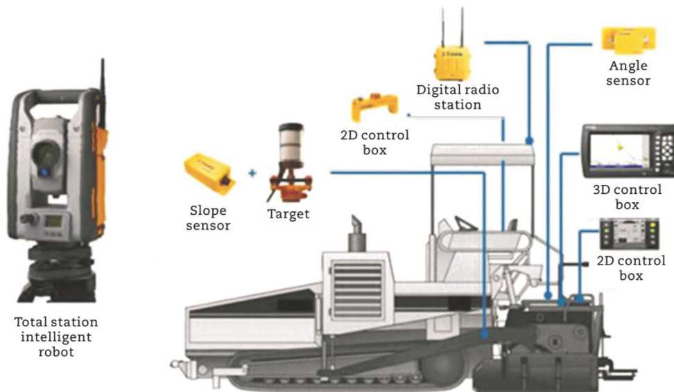
Fig. 69. 3D paving system composition.
