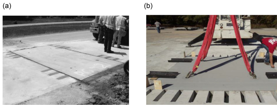
Fig. 54. Typical applications of the Michigan slab system. (a) Repairing road. (b) Repairing airport pavement.
