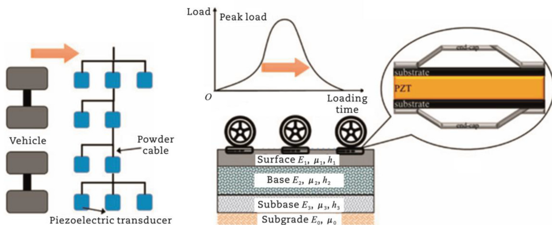
Fig. 2. Piezoelectric integration schematic (Wang et al., 2021d).
