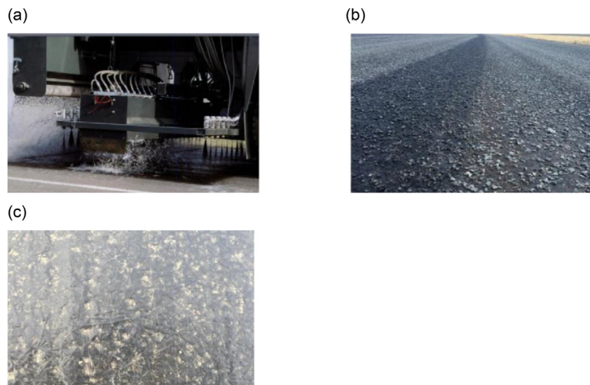
Fig. 40. Field application of fiber chip seal technology. (a) Paving construction. (b) Curing. (c) Open to traffic (Vargas-Nordbeck and Jalali, 2020; Nair and McGhee, 2022).
