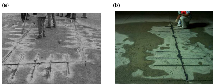
Fig. 55. Typical application of Uretek stitch slab system. (a) Repairing the pavement. (b) Reinforcing the road.
