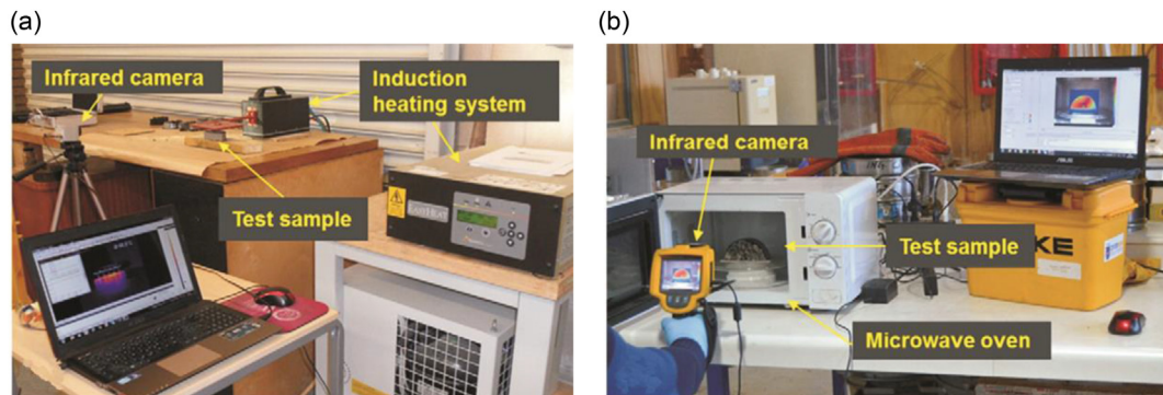
Fig. 10. Thermal induced healing technology. (a) Electromagnetic induction heating healing. (b) Microwave induction heating healing (Norambuena-Contreras and Garcia, 2016).
