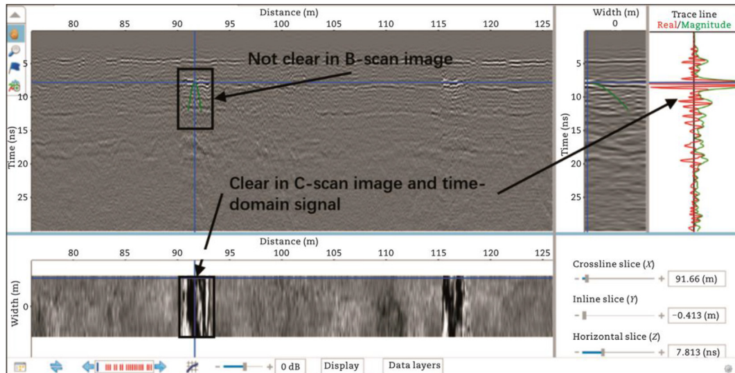
Fig. 87. Small object detection using B- and C-scan imaging.
