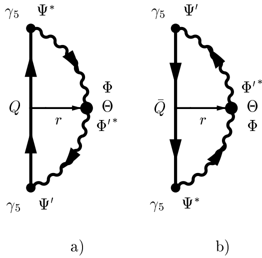
FIG. 2. The two contributions to the three-point correlation function C_3
