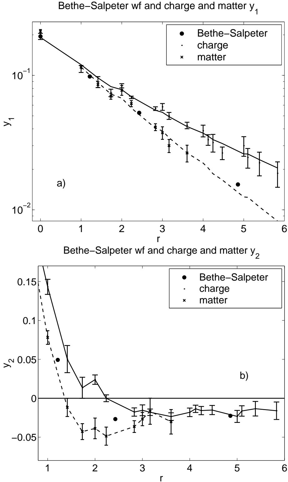
FIG. 5. The separable "wavefunctions" y_1 and y_2 defined in the density x^{\alpha\beta}(r) = y_\alpha(r)y_\beta(r) . a) y_1 — Solid line for the charge, dashed for the matter, solid circles the Bethe-Salpeter wavefunction from Ref. [5], b) y_2 — notation as in a)
