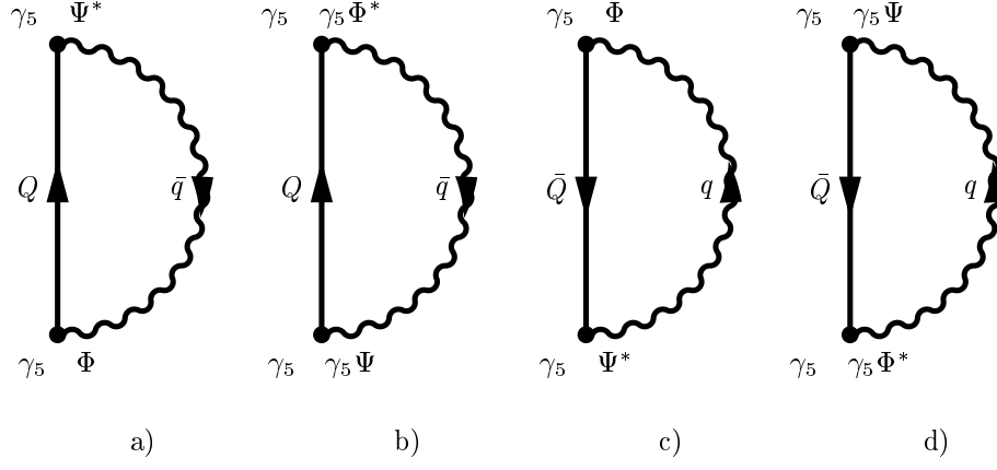
FIG. 1. The four contributions to the two-point correlation function C_2
