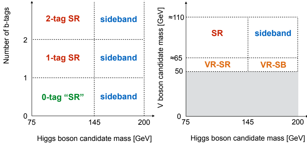
Figure 1: Illustration of the sideband and validation regions, showing orthogonal slices through the space defined by the masses of the two boson candidates and the number of b -tags.
