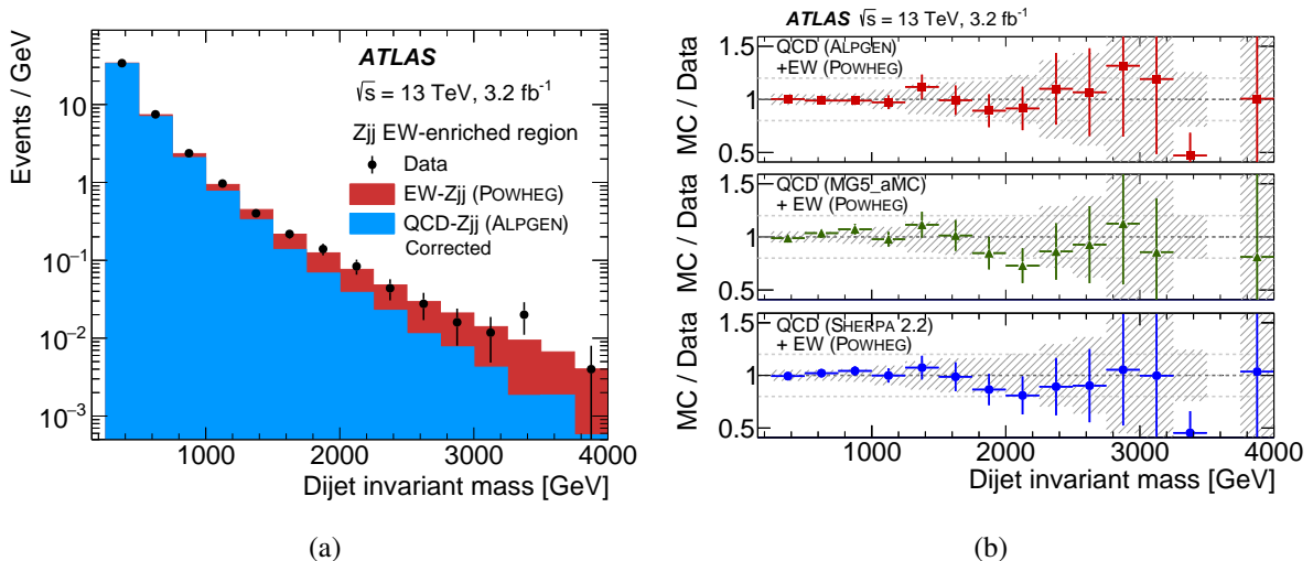
Figure 4: (a) Comparison in the EW-enriched region of the sum of EW-Z _{jj} and m_{jj} -reweighted QCD-Z _{jj} templates to the data (minus the non-Z _{jj} backgrounds). The normalisation of the templates is adjusted to the results of the fit (see text for details). The EW-Z _{jj} MC sample comes from the POWHEG event generator and the QCD-Z _{jj} MC sample comes from the ALPGEN event generator. (b) The ratio of the sum of the EW-Z _{jj} and m_{jj} -reweighted QCD-Z _{jj} templates to the background-subtracted data in the EW-enriched region, for three different QCD-Z _{jj} MC predictions. The normalisation of the templates is adjusted to the results of the fit. Error bars represent the statistical uncertainties in the data and combined QCD-Z _{jj} plus EW-Z _{jj} MC samples added in quadrature. The hatched band represents experimental systematic uncertainties in the m_{jj} distribution.
