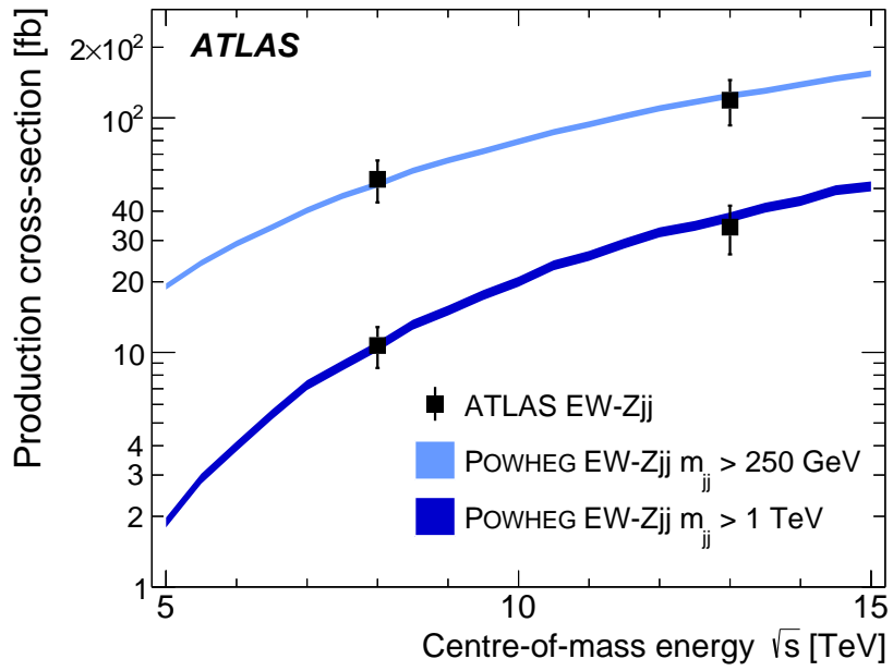
Figure 6: Measurements of the EW-Zjj process presented in this Letter at a centre-of-mass energy of 13 TeV, compared with previous measurements at 8 TeV [1], for two different dijet invariant mass thresholds, m_{jj} > 0.25 TeV and m_{jj} > 1 TeV. The error bars on the measurements represent statistical and systematic uncertainties added in quadrature. Predictions from the POWHEG event generator with their total uncertainty are also shown.
