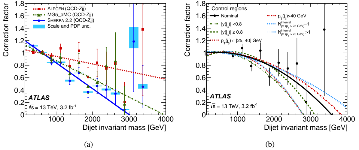
Figure 3: Binned data-to-simulation normalised ratio shape correction factors as a function of dijet invariant mass in the QCD-enriched region. (a) Ratio for three different QCD- Z_{jj} MC samples with uncertainties corresponding to the combined statistical uncertainties in the data and QCD- Z_{jj} MC samples added in quadrature. Scale and PDF uncertainties in SHERPA predictions are indicated by the shaded bands. Lines represent fits to the ratios using a linear fit. (b) Ratio for subregions of the QCD-enriched region for the ALPGEN MC sample. Curves represent the result of fits with a quadratic function for the various subregions.
