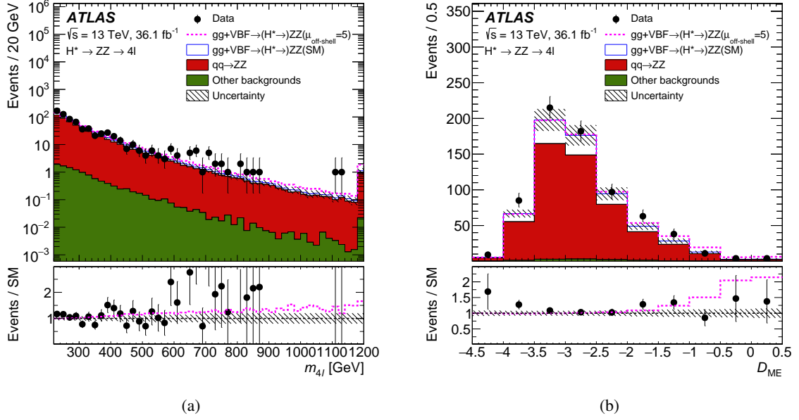
Figure 1: Observed distributions in the range 220 \text{ GeV} < m_{4\ell} < 2000 \text{ GeV} for (a) the four-lepton invariant mass m_{4\ell} and (b) the ME-based discriminant D_{ME} combining all lepton final states, compared to the expected contributions from the SM including the Higgs boson (stacked). Events with m_{4\ell} > 1200 \text{ GeV} are included in the last bin of the m_{4\ell} distribution. The hatched area shows the combined statistical and systematic uncertainties. The dashed line corresponds to the total expected event yield, including all backgrounds and the Higgs boson with \mu_{\text{off-shell}} = 5 . The ratio plot shows the observed data yield divided by the SM prediction (black points) as well as the total expected event yield with \mu_{\text{off-shell}} = 5 divided by the SM prediction (dashed line) in each bin.
